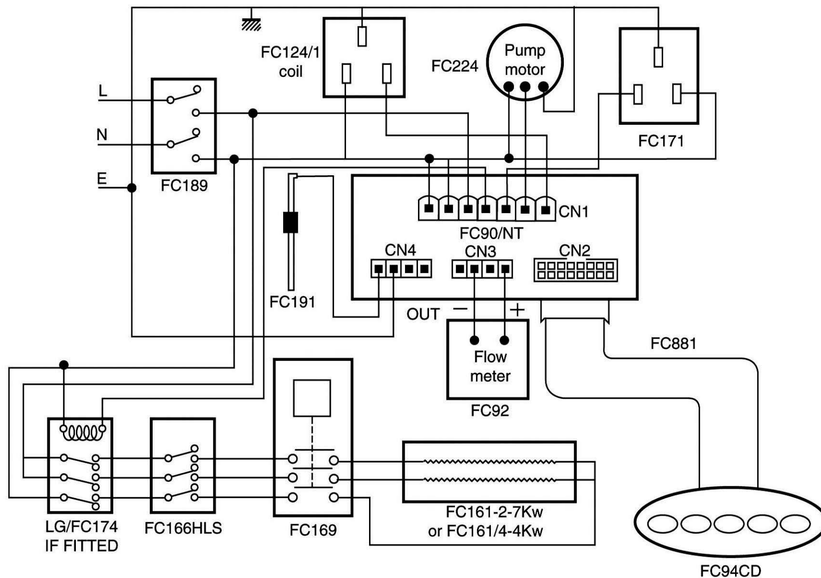
CIRCUIT DIAGRAM
